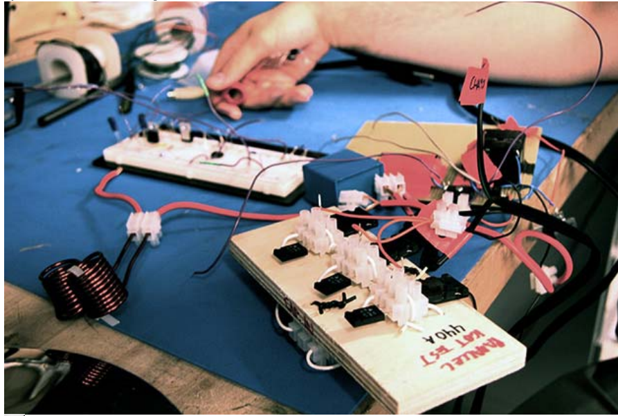
Dr. Ed Boyden displays the small prototype Transcranial Magnetic Stimulation machine built by his students at the Neuroengineering and Neuromedia Lab at MIT. The copper coils generate magnetic fields that creates a current in adjacent brain tissue.
